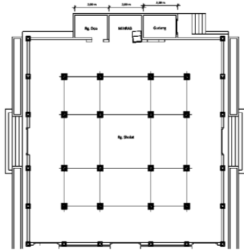
1 DENAH MASJID A01 Scale: 1 : 100
