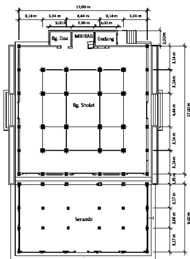
Gambar Denah Masjid Ki Mageti
