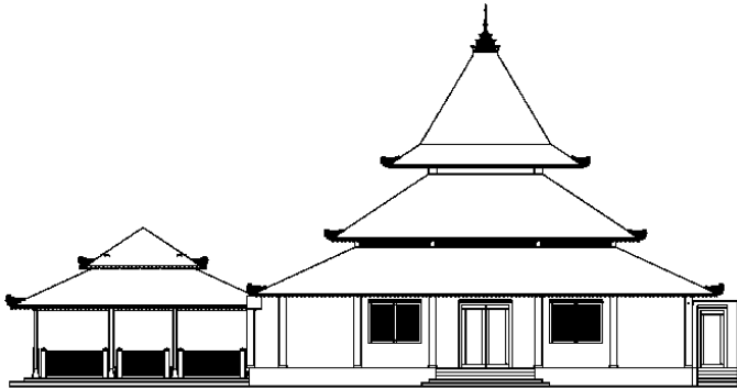
1 TAMPAK UTARA A/B/C D/G/H/I Scale: 1 : 100
